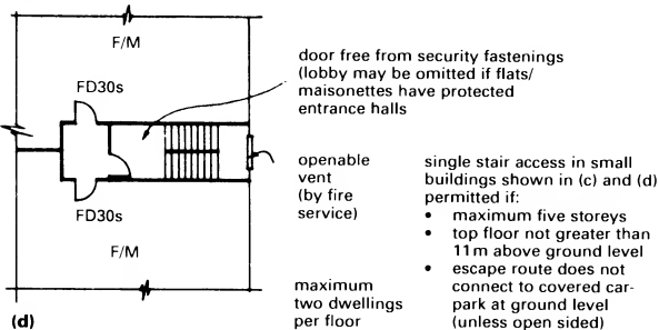
① Typical arrangements for flats or maisonettes with single common stairs according to the Building Regulations for England and Wales: (a) corridor access, (b) lobby access, (c) and (d) single stair access in small buildings
